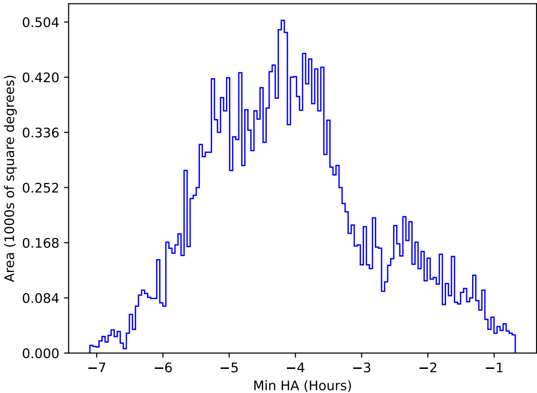
too_elab_heavy_r64_d3_griz_v3.4_10yrs All sky z band: Min HA
