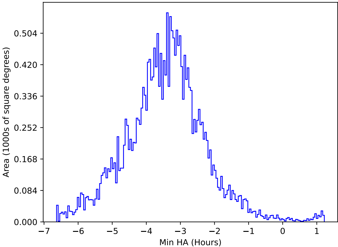
too_elab_heavy_r64_d3_griz_v3.4_10yrs All sky y band: Min HA
