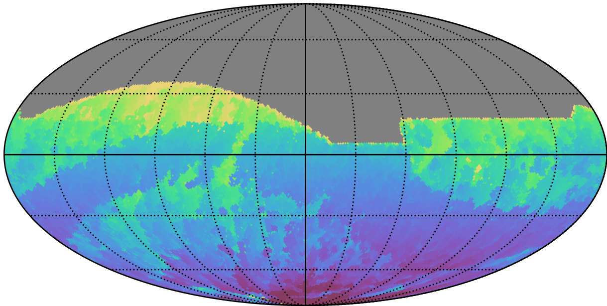
too_elab_heavy_r64_d3_griz_v3.4_10yrs All sky r band: Min HA
