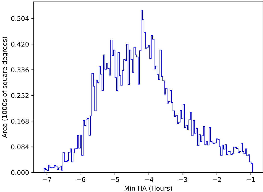
too_elab_heavy_r64_d3_griz_v3.4_10yrs All sky r band: Min HA
