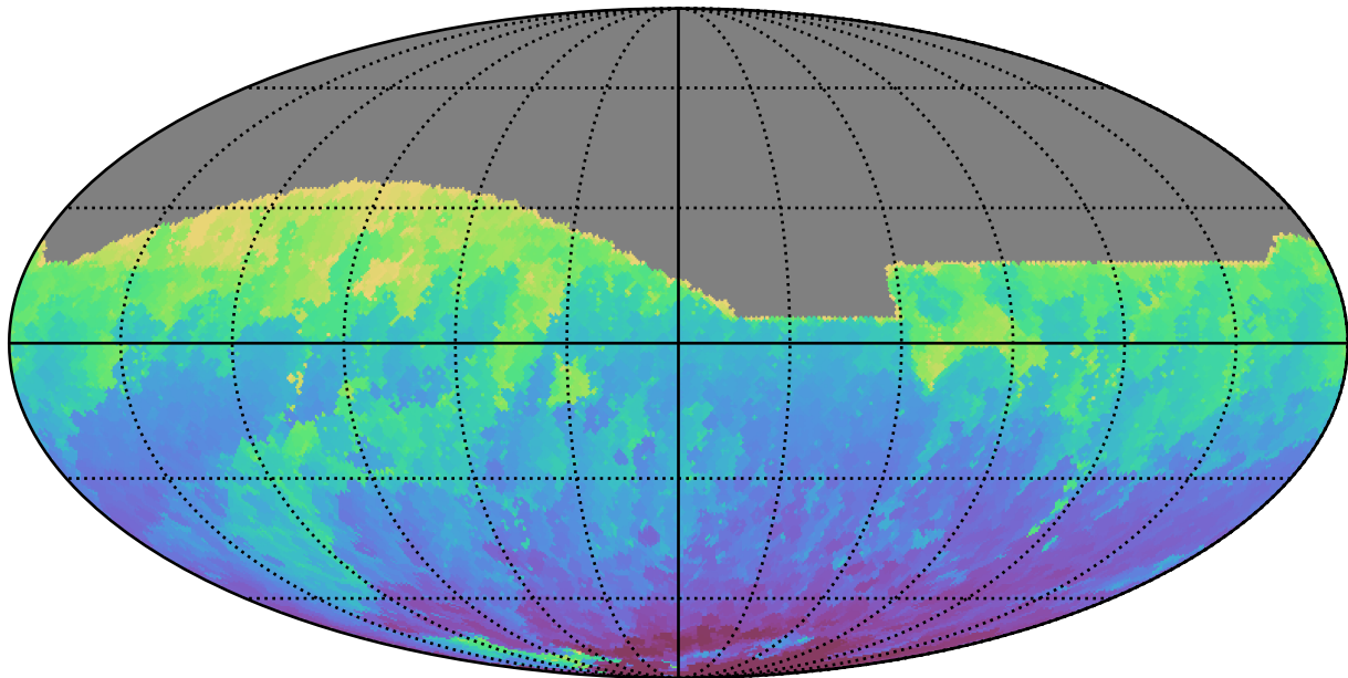
too_elab_heavy_r64_d3_griz_v3.4_10yrs All sky i band: Min HA
