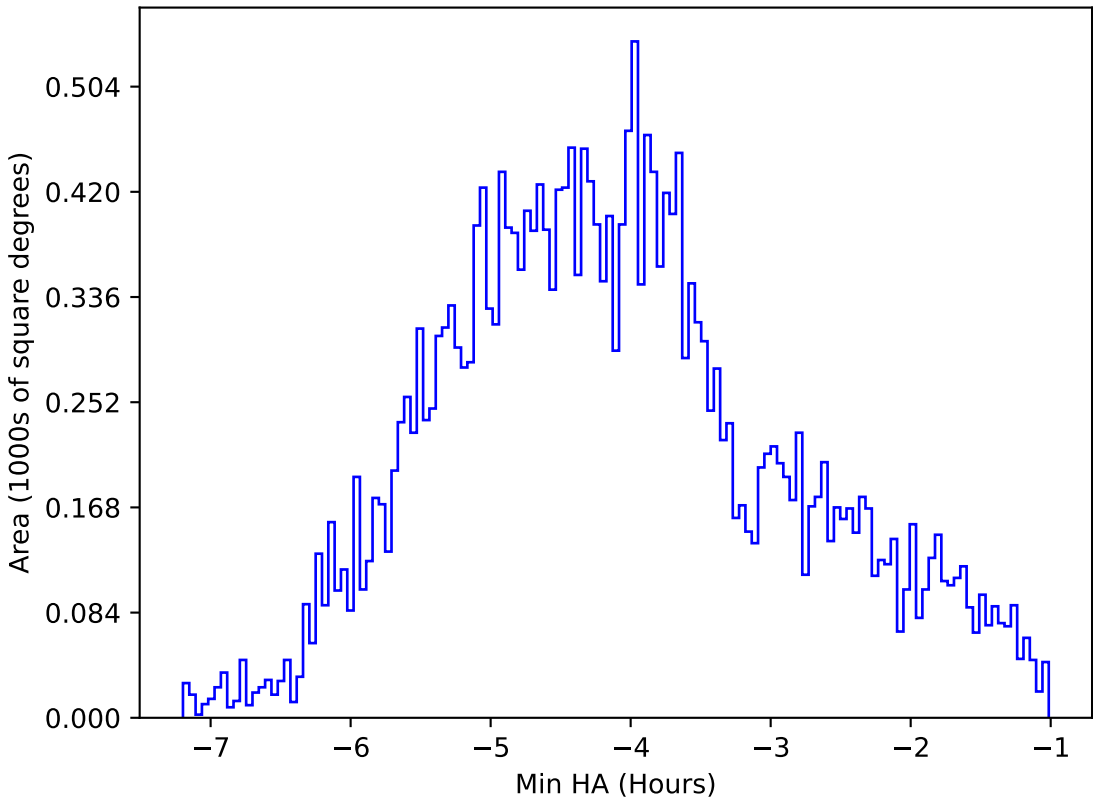
too_elab_heavy_r64_d3_griz_v3.4_10yrs All sky i band: Min HA
