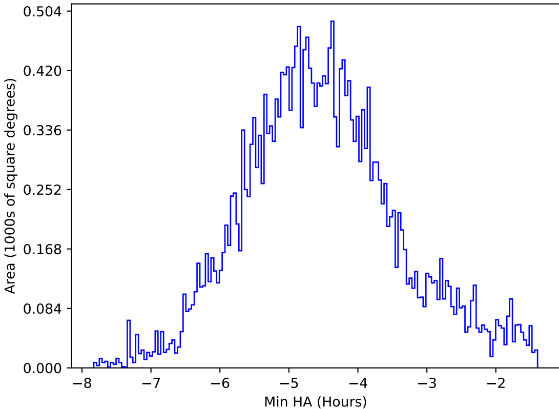
too_elab_heavy_r64_d3_griz_v3.4_10yrs All sky all bands: Min HA
