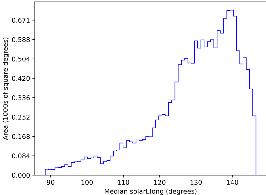
too_elab_heavy_r64_d3_griz_v3.4_10yrs WFD all bands: Median solarElong
