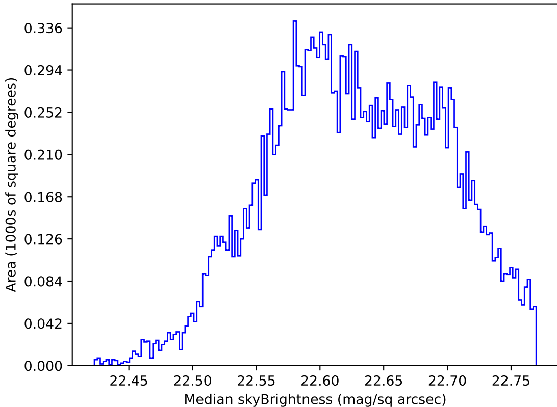
too_elab_heavy_r64_d3_griz_v3.4_10yrs Yr 1 u band: Median skyBrightness
