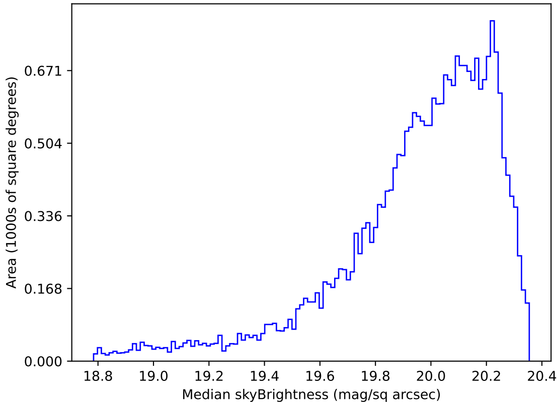
too_elab_heavy_r64_d3_griz_v3.4_10yrs Yr 1 i band: Median skyBrightness
