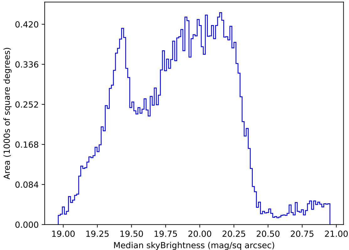
too_elab_heavy_r64_d3_griz_v3.4_10yrs Yr 1 all bands: Median skyBrightness
