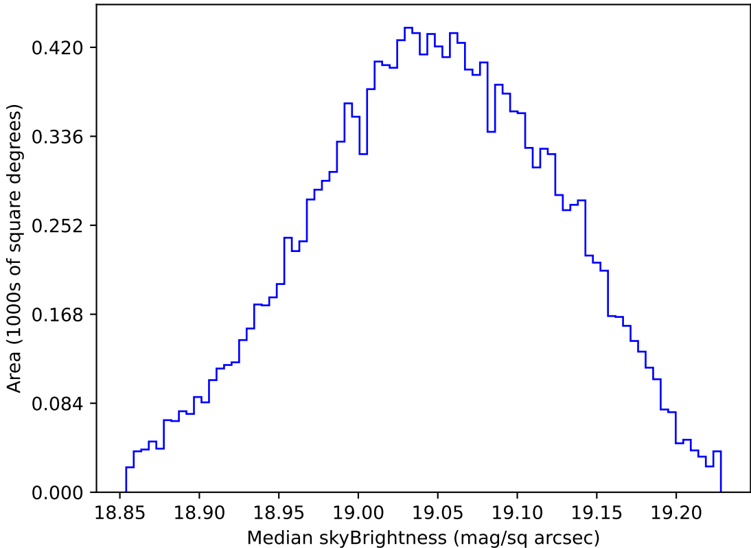
too_elab_heavy_r64_d3_griz_v3.4_10yrs WFD z band: Median skyBrightness
