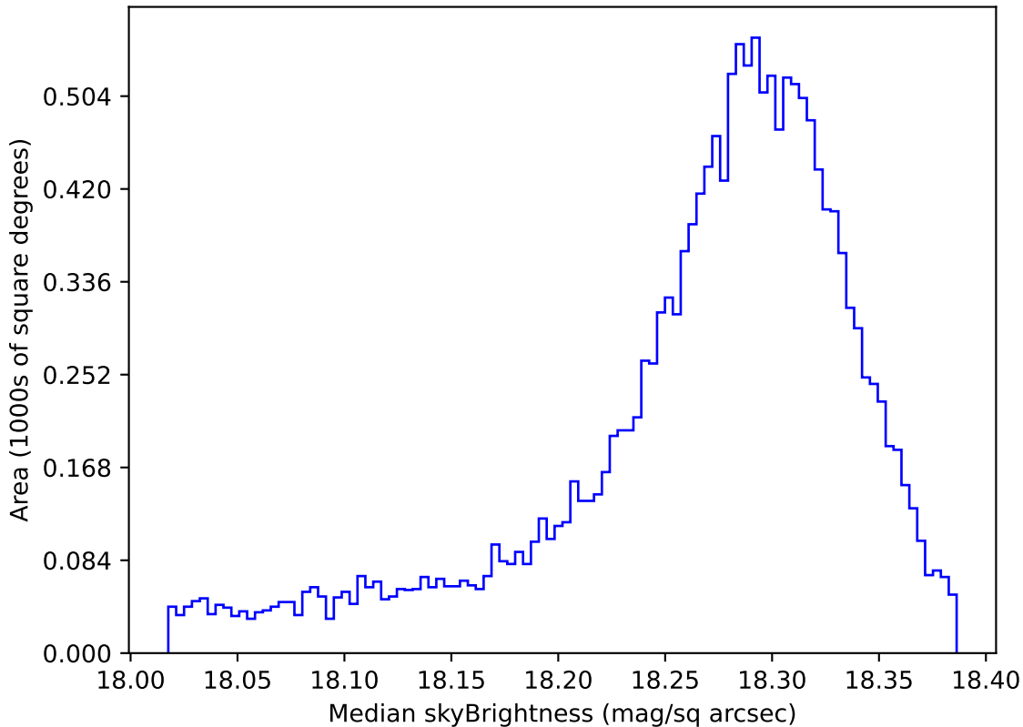
too_elab_heavy_r64_d3_griz_v3.4_10yrs WFD y band: Median skyBrightness
