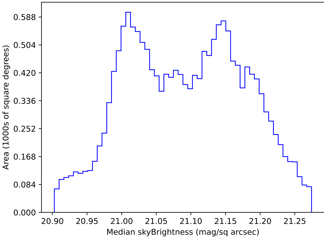
too_elab_heavy_r64_d3_griz_v3.4_10yrs WFD r band: Median skyBrightness
