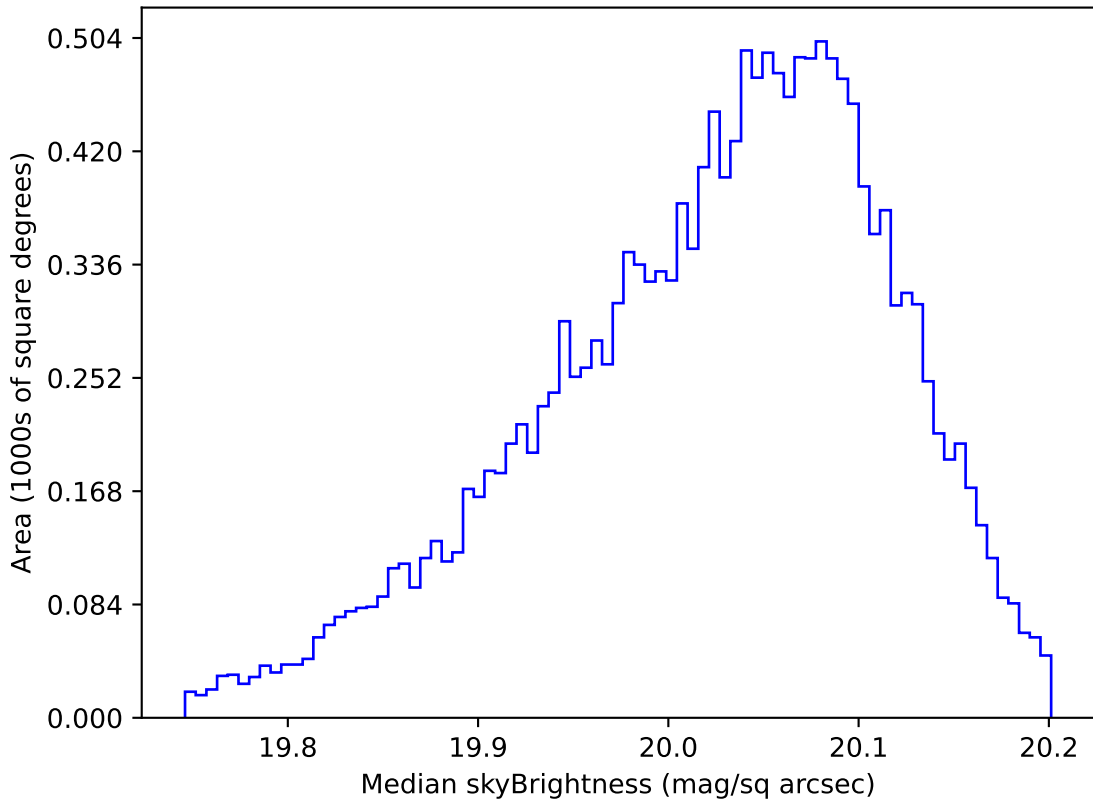
too_elab_heavy_r64_d3_griz_v3.4_10yrs WFD i band: Median skyBrightness
