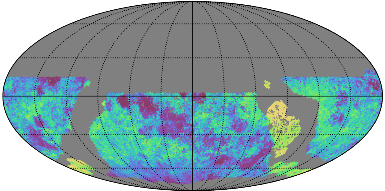
too_elab_heavy_r64_d3_griz_v3.4_10yrs WFD all bands: Median skyBrightness
