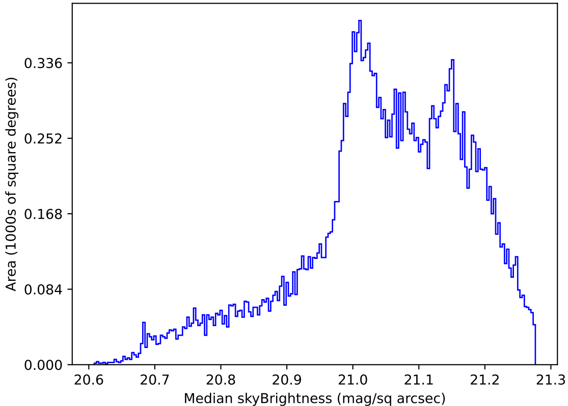
too_elab_heavy_r64_d3_griz_v3.4_10yrs All sky r band: Median skyBrightness
