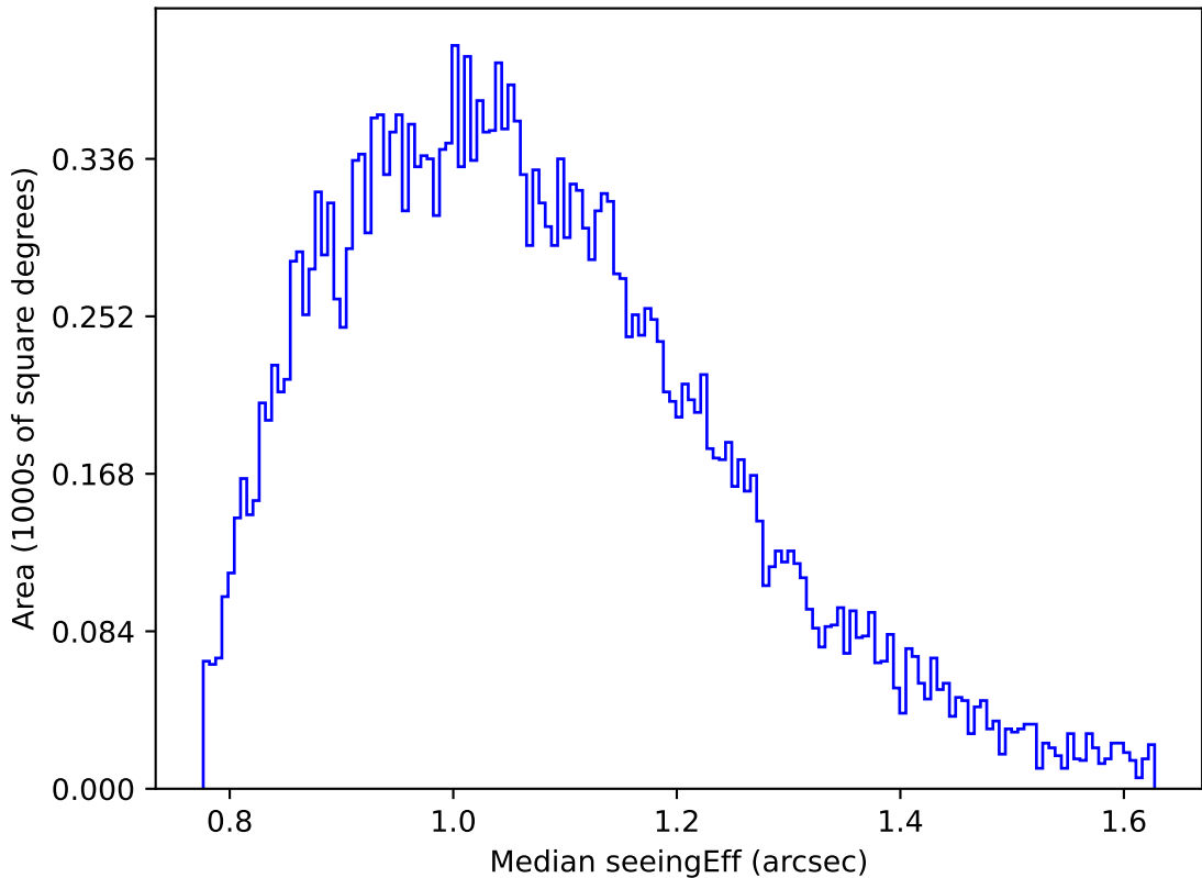
too_elab_heavy_r64_d3_griz_v3.4_10yrs Yr 1 g band: Median seeingEff
