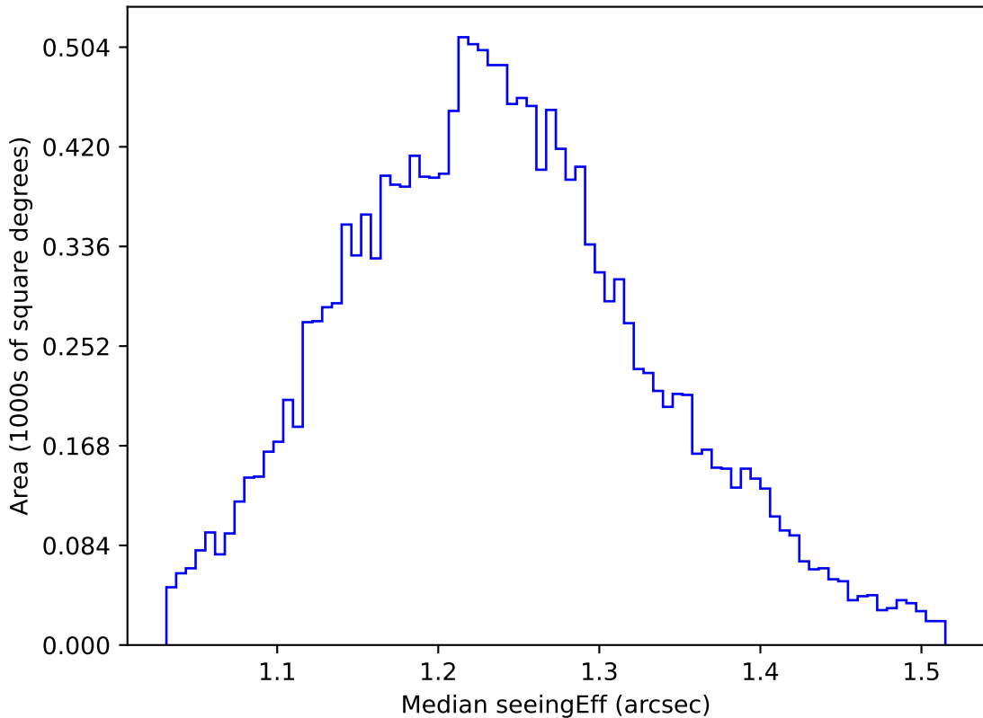
too_elab_heavy_r64_d3_griz_v3.4_10yrs WFD u band: Median seeingEff
