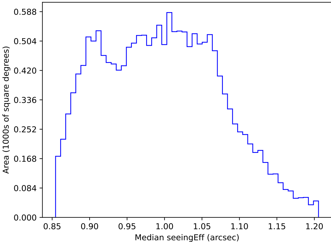
too_elab_heavy_r64_d3_griz_v3.4_10yrs WFD i band: Median seeingEff
