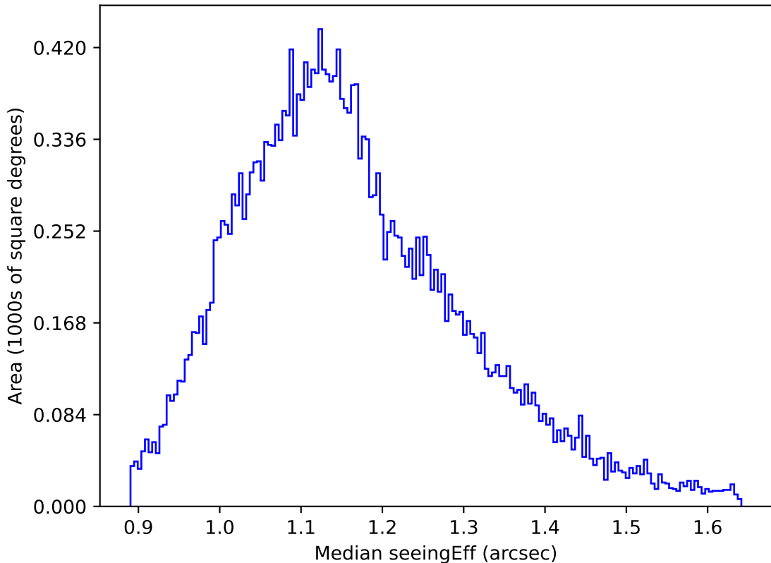
too_elab_heavy_r64_d3_griz_v3.4_10yrs All sky g band: Median seeingEff
