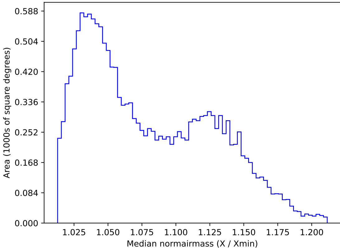
too_elab_heavy_r64_d3_griz_v3.4_10yrs WFD u band: Median normairmass
