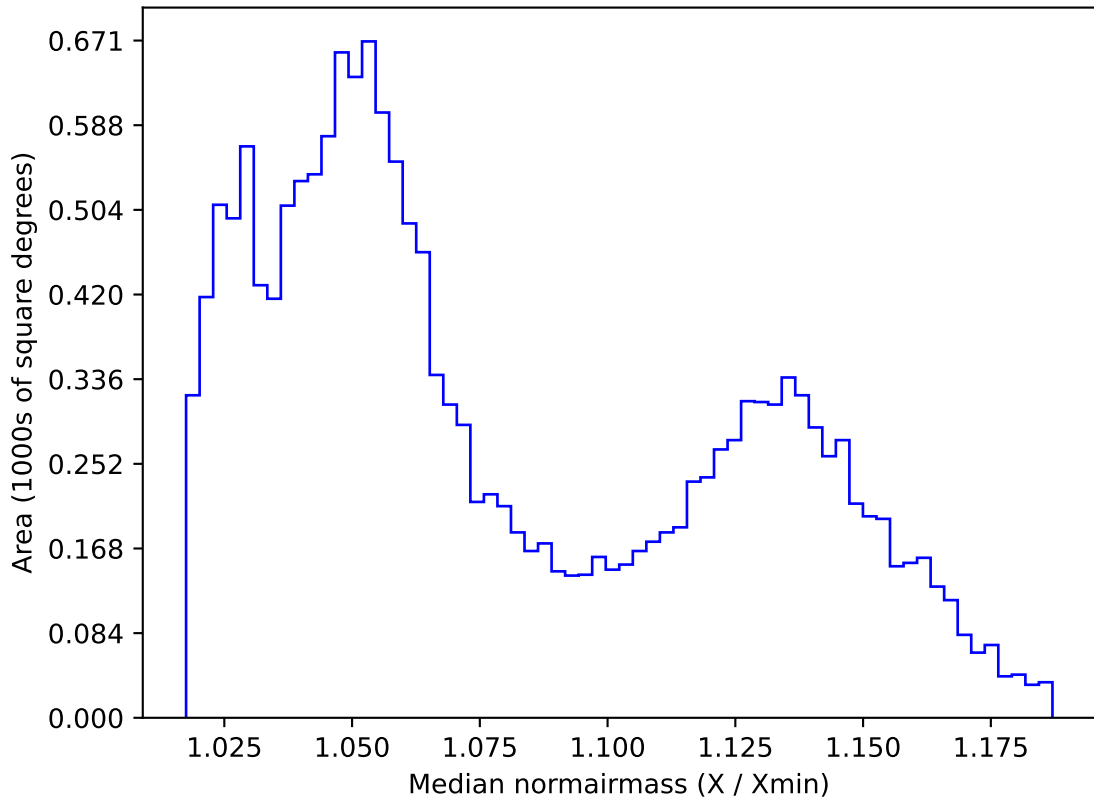
too_elab_heavy_r64_d3_griz_v3.4_10yrs WFD r band: Median normairmass
