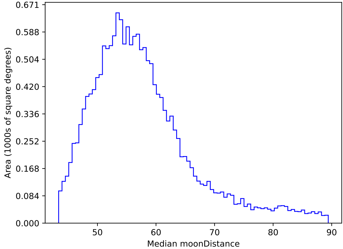
too_elab_heavy_r64_d3_griz_v3.4_10yrs WFD y band: Median moonDistance
