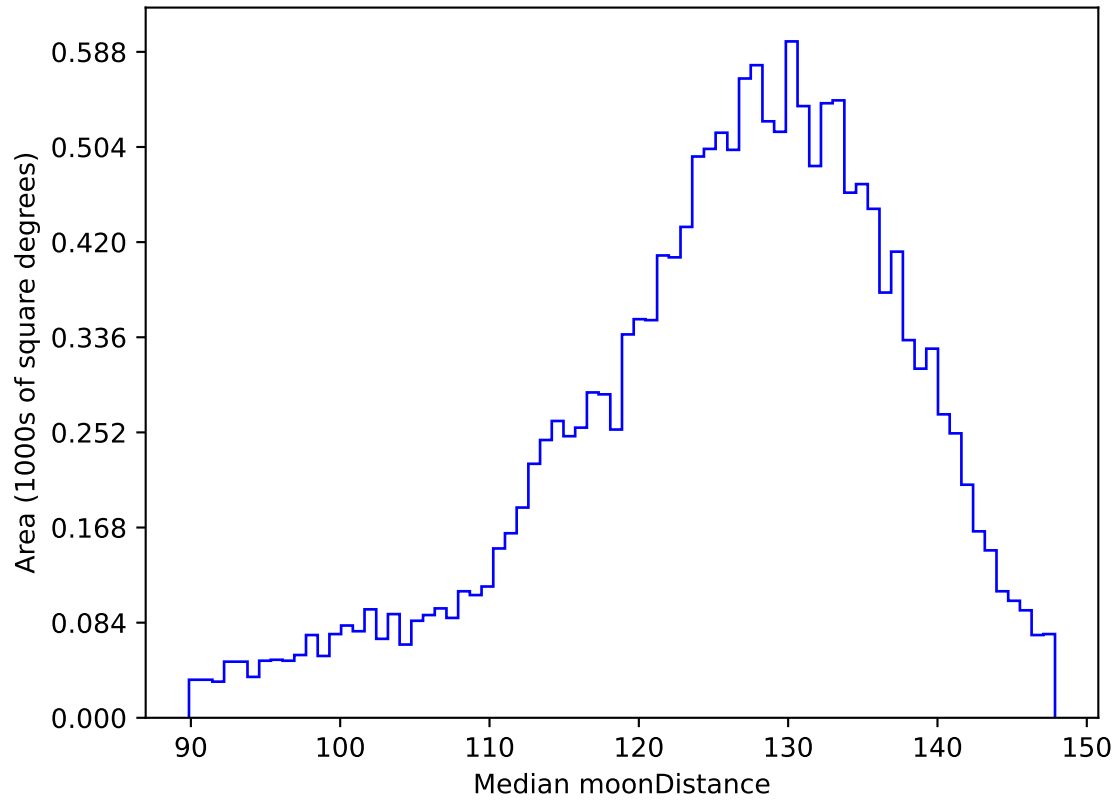
too_elab_heavy_r64_d3_griz_v3.4_10yrs WFD u band: Median moonDistance
