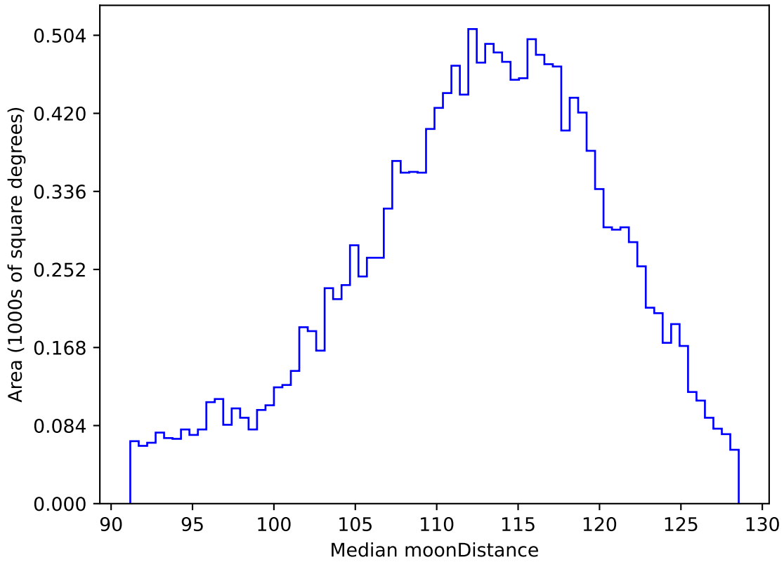
too_elab_heavy_r64_d3_griz_v3.4_10yrs WFD r band: Median moonDistance
