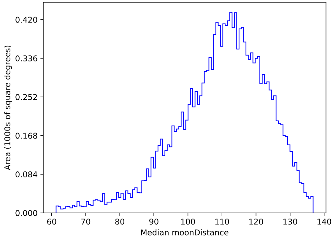
too_elab_heavy_r64_d3_griz_v3.4_10yrs WFD g band: Median moonDistance
