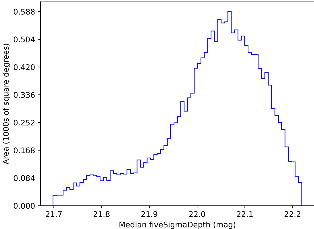
too_elab_heavy_r64_d3_griz_v3.4_10yrs WFD y band: Median fiveSigmaDepth
