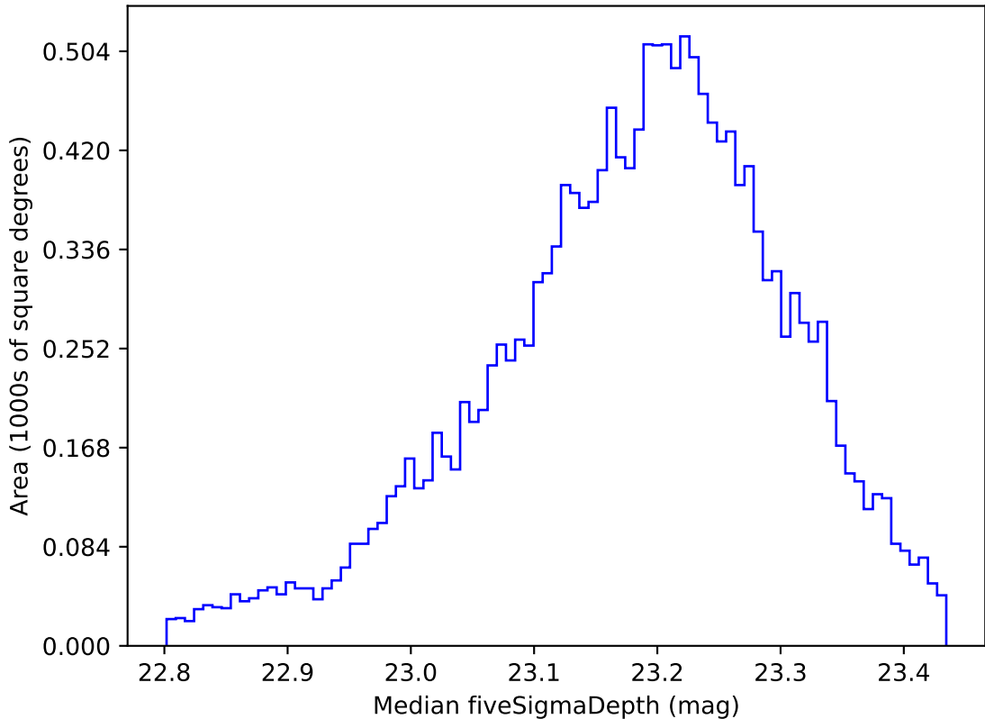
too_elab_heavy_r64_d3_griz_v3.4_10yrs WFD u band: Median fiveSigmaDepth
