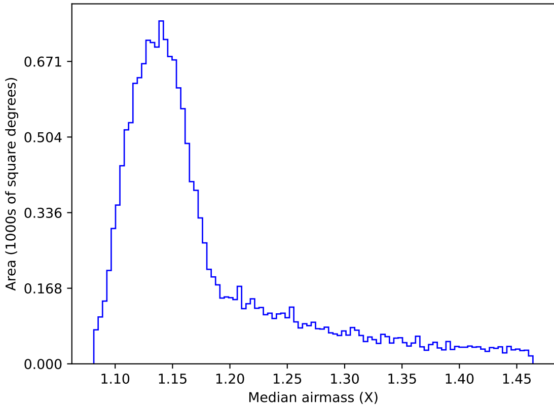
too_elab_heavy_r64_d3_griz_v3.4_10yrs WFD i band: Median airmass
