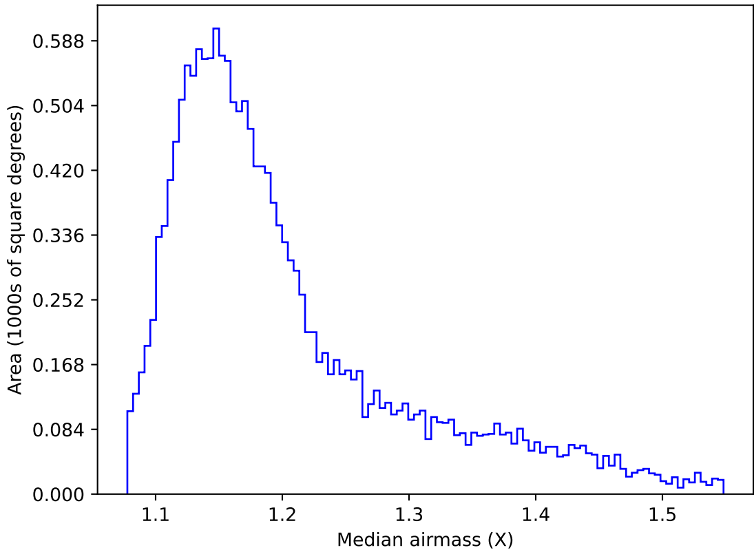
too_elab_heavy_r64_d3_griz_v3.4_10yrs WFD g band: Median airmass
