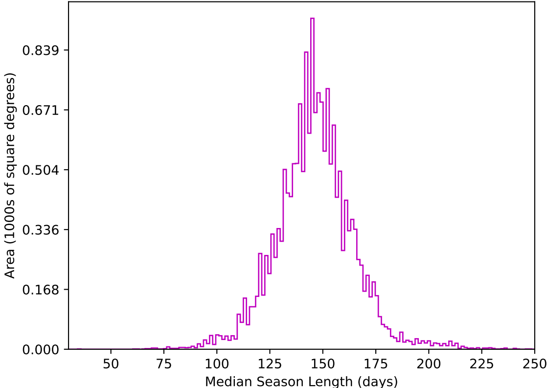
too_elab_heavy_r64_d3_griz_v3.4_10yrs WFD z band: Median Season Length
