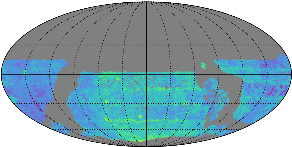
too_elab_heavy_r64_d3_griz_v3.4_10yrs WFD y band: Median Season Length
