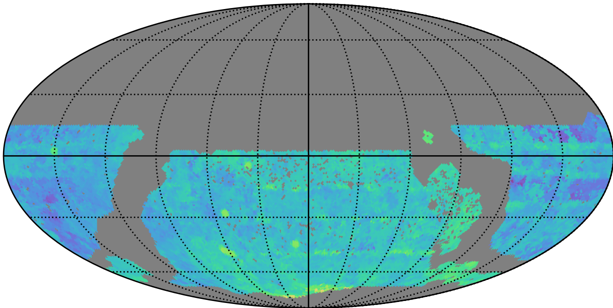
too_elab_heavy_r64_d3_griz_v3.4_10yrs WFD i band: Median Season Length
