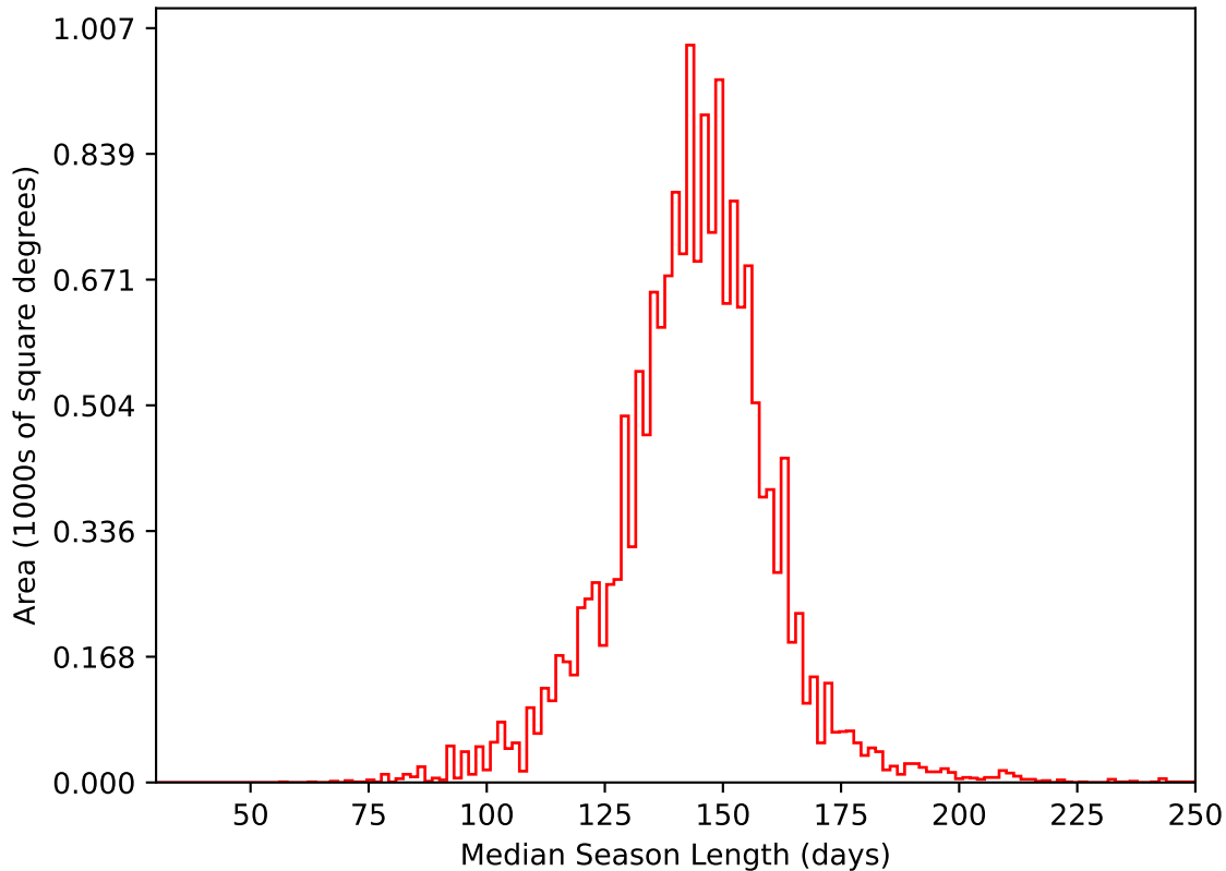
too_elab_heavy_r64_d3_griz_v3.4_10yrs WFD i band: Median Season Length
