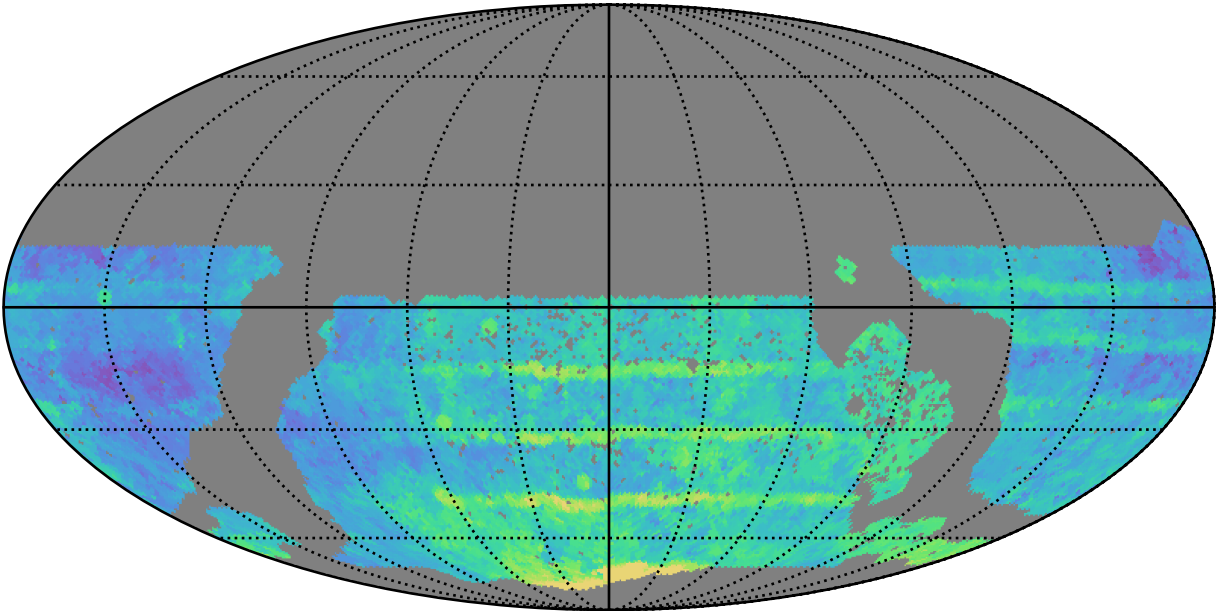
too_elab_heavy_r64_d3_griz_v3.4_10yrs WFD all bands: Median Season Length
