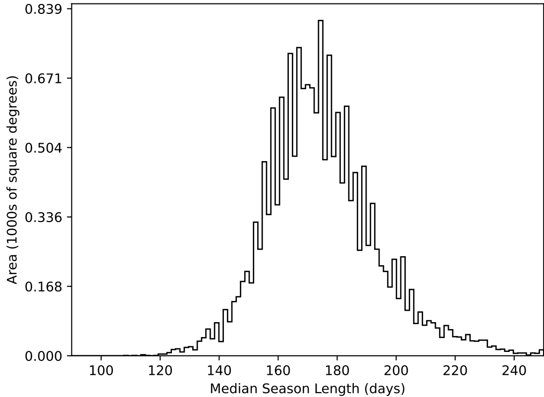
too_elab_heavy_r64_d3_griz_v3.4_10yrs WFD all bands: Median Season Length
