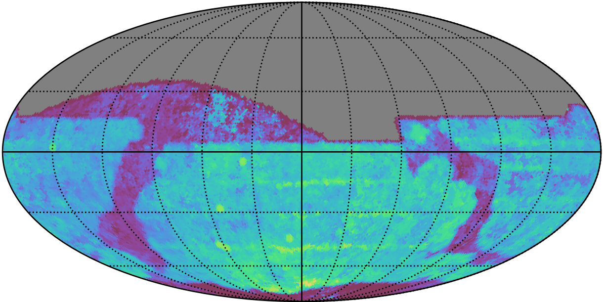
too_elab_heavy_r64_d3_griz_v3.4_10yrs All sky z band: Median Season Length
