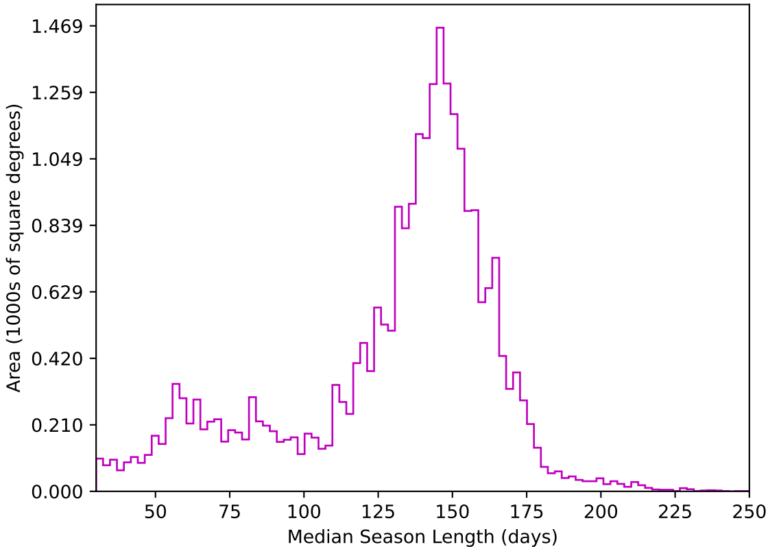
too_elab_heavy_r64_d3_griz_v3.4_10yrs All sky z band: Median Season Length
