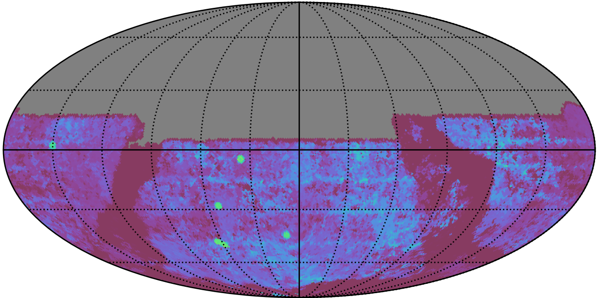
too_elab_heavy_r64_d3_griz_v3.4_10yrs All sky u band: Median Season Length
