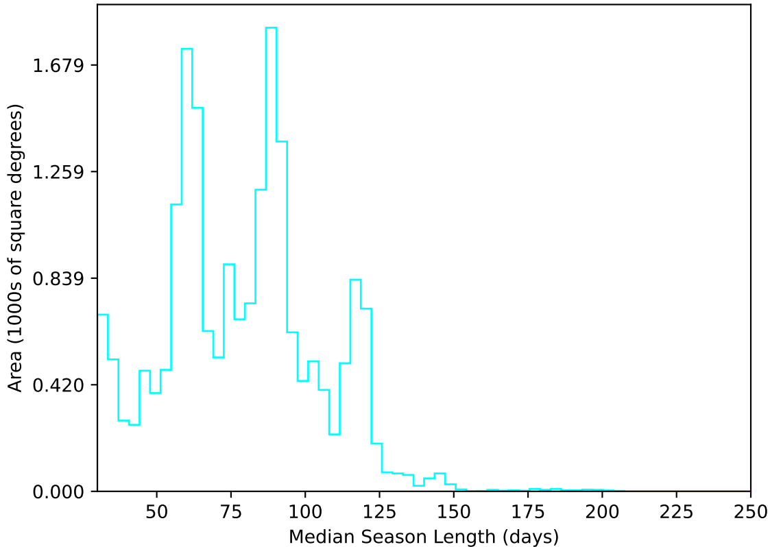
too_elab_heavy_r64_d3_griz_v3.4_10yrs All sky u band: Median Season Length
