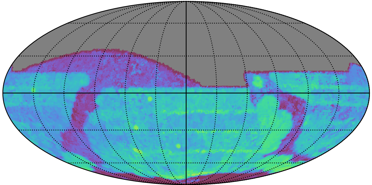
too_elab_heavy_r64_d3_griz_v3.4_10yrs All sky r band: Median Season Length
