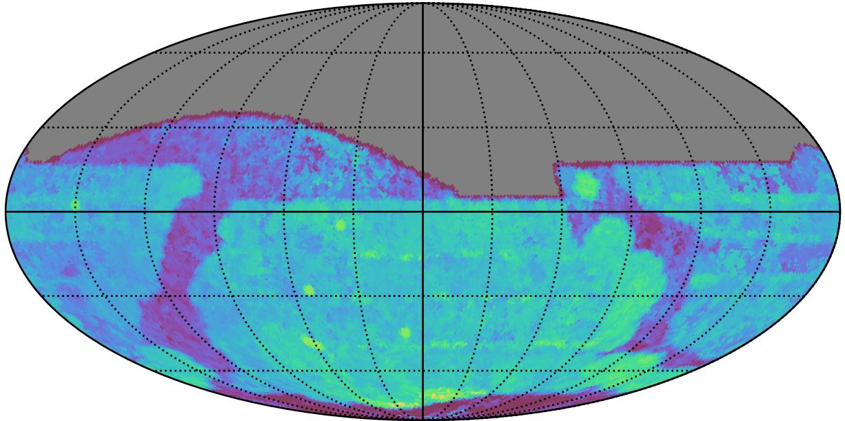
too_elab_heavy_r64_d3_griz_v3.4_10yrs All sky i band: Median Season Length
