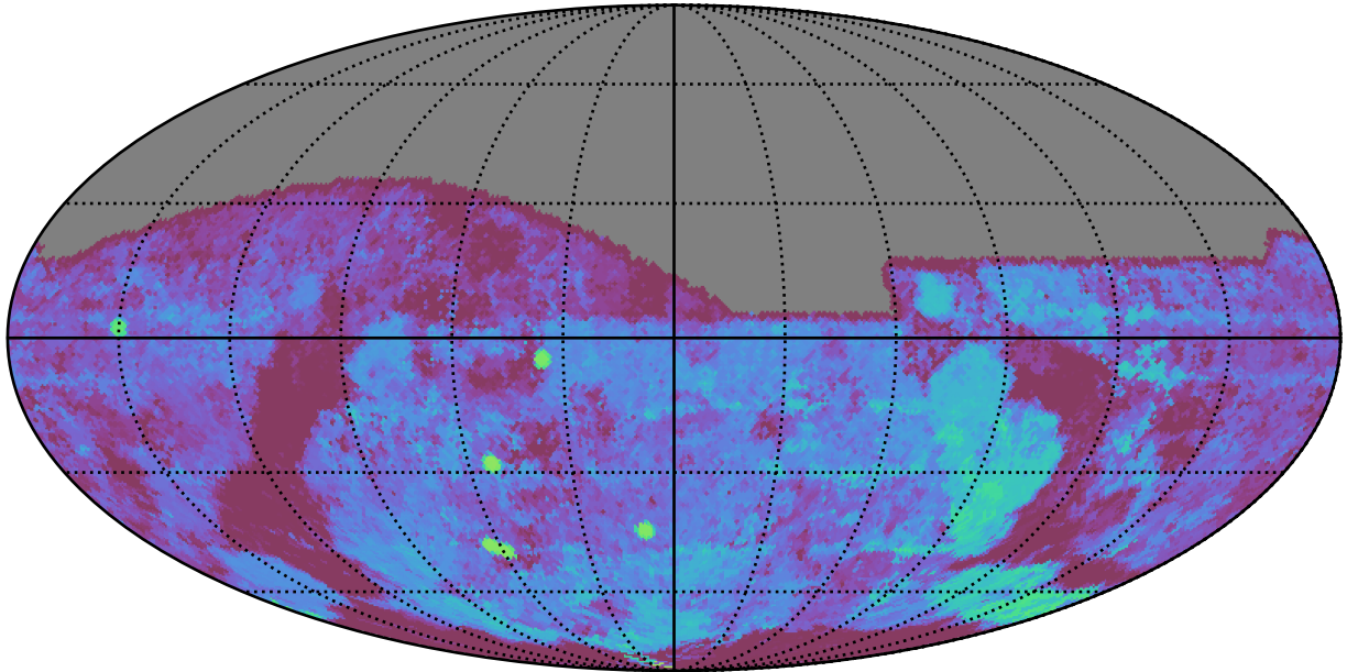
too_elab_heavy_r64_d3_griz_v3.4_10yrs All sky g band: Median Season Length
