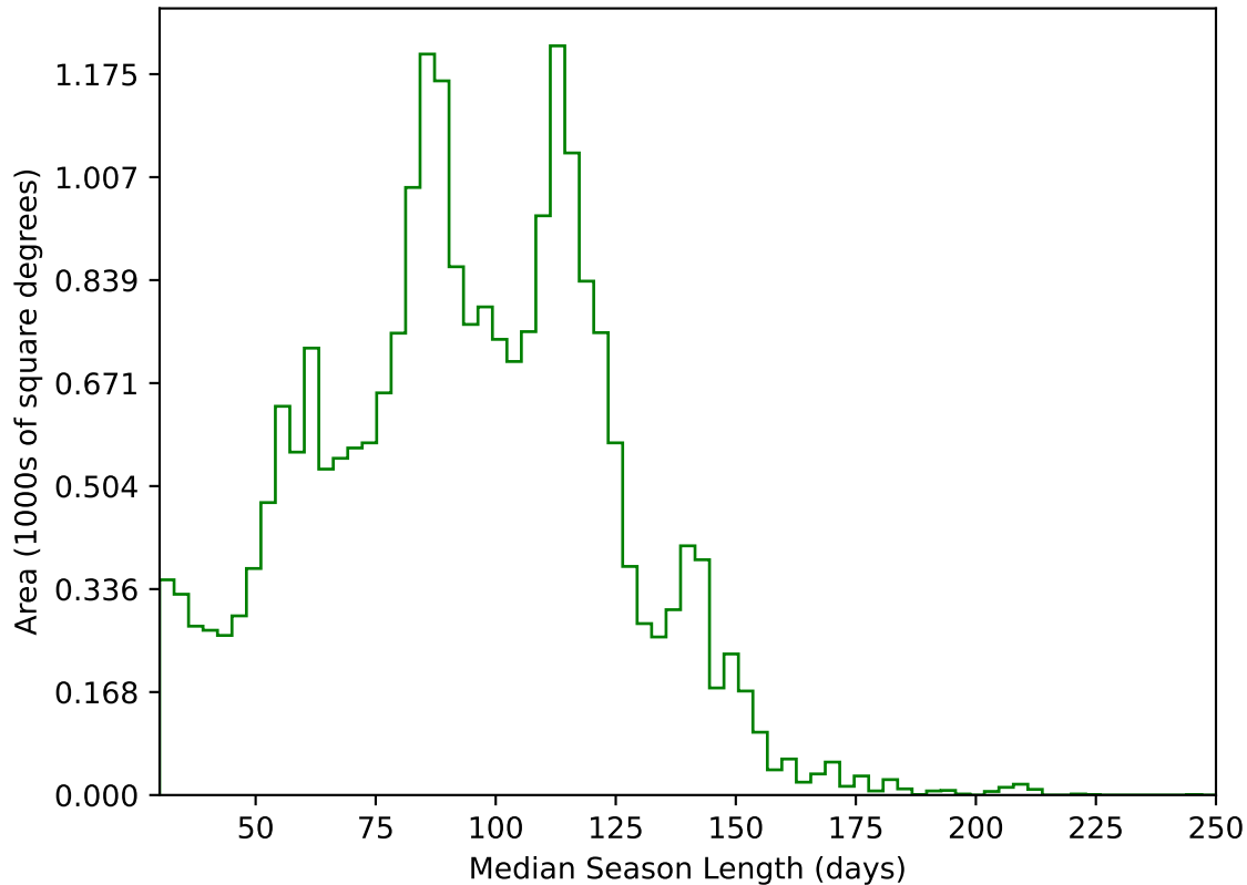
too_elab_heavy_r64_d3_griz_v3.4_10yrs All sky g band: Median Season Length
