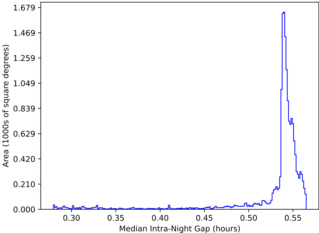
too_elab_heavy_r64_d3_griz_v3.4_10yrs WFD: Median Intra-Night Gap
