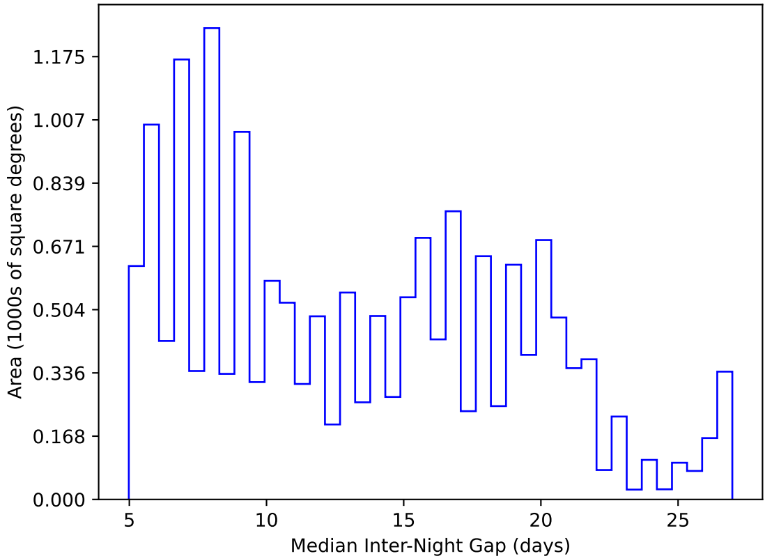
too_elab_heavy_r64_d3_griz_v3.4_10yrs WFD y band: Median Inter-Night Gap
