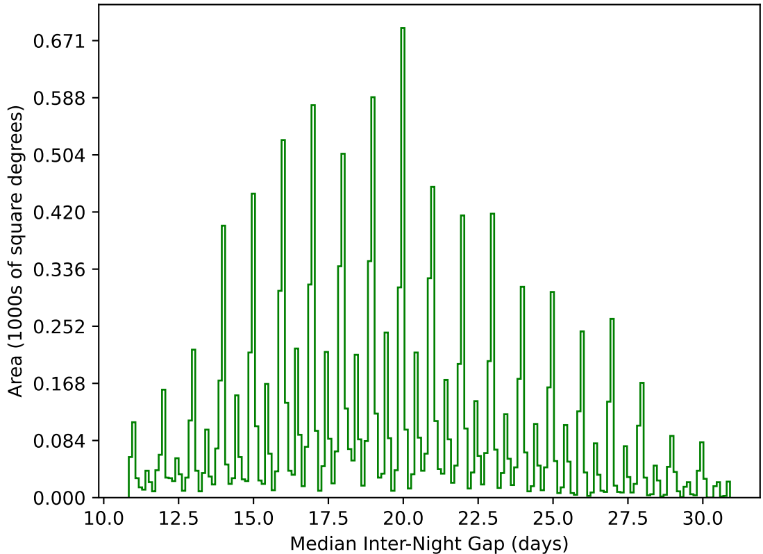
too_elab_heavy_r64_d3_griz_v3.4_10yrs WFD g band: Median Inter-Night Gap
