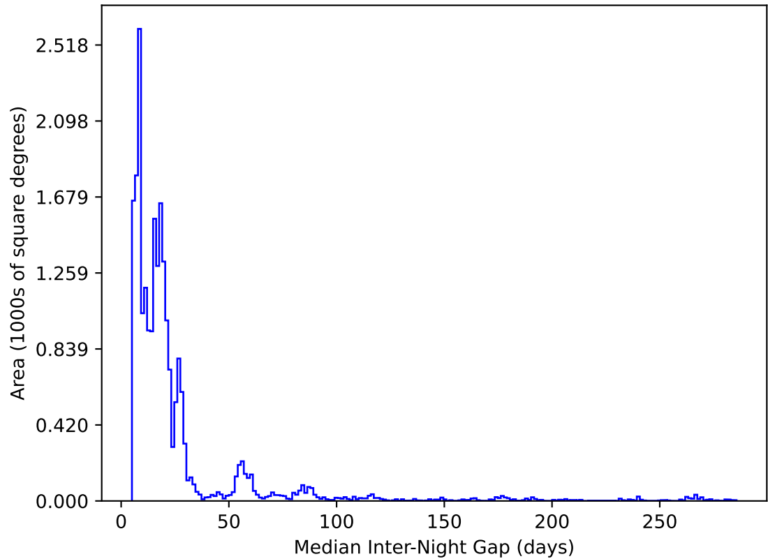
too_elab_heavy_r64_d3_griz_v3.4_10yrs All sky y band: Median Inter-Night Gap
