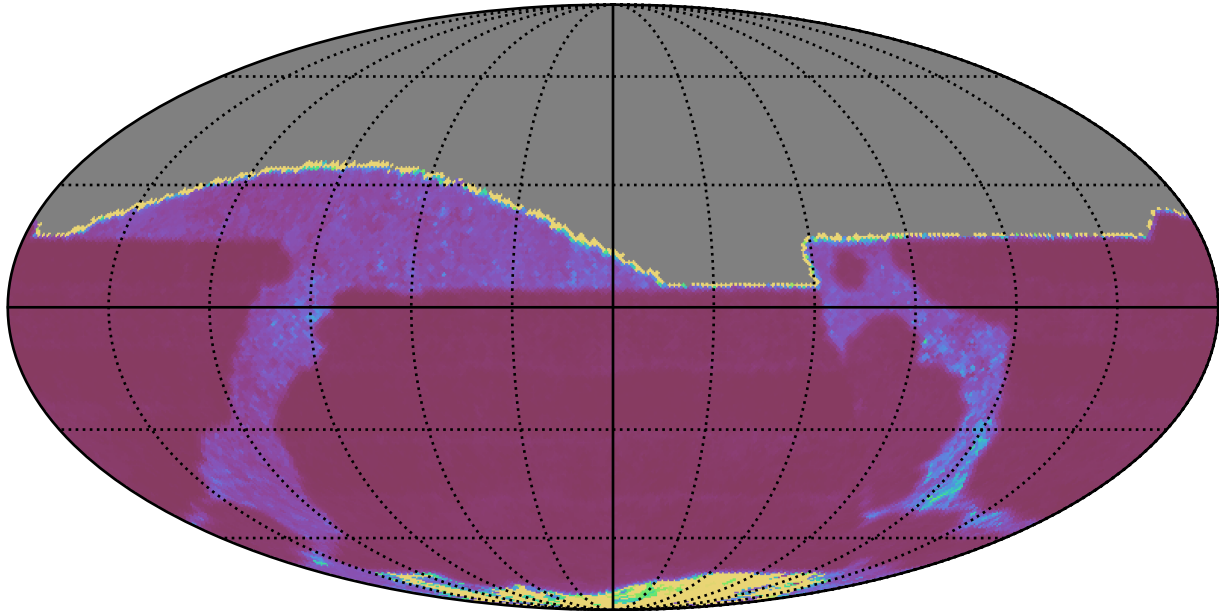
too_elab_heavy_r64_d3_griz_v3.4_10yrs All sky r band: Median Inter-Night Gap
